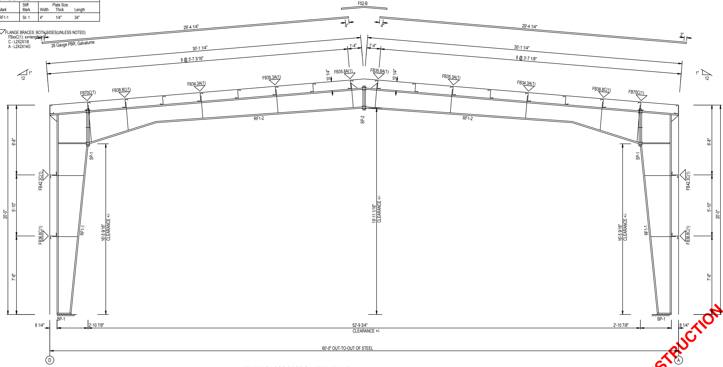
FRAME CROSS SECTION: FRAME LINE 2 3 4 5
