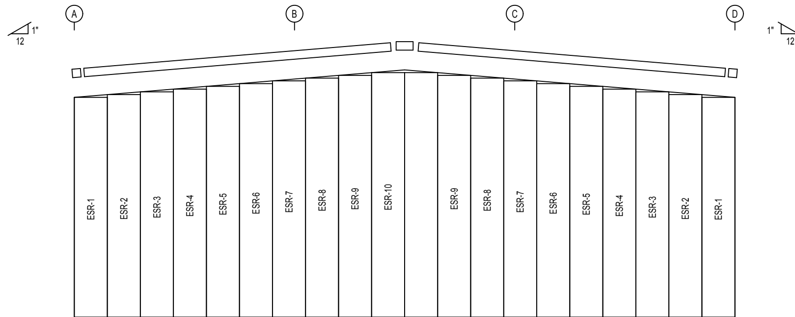
ENDWALL SHEETING & TRIM: FRAME LINE 6
