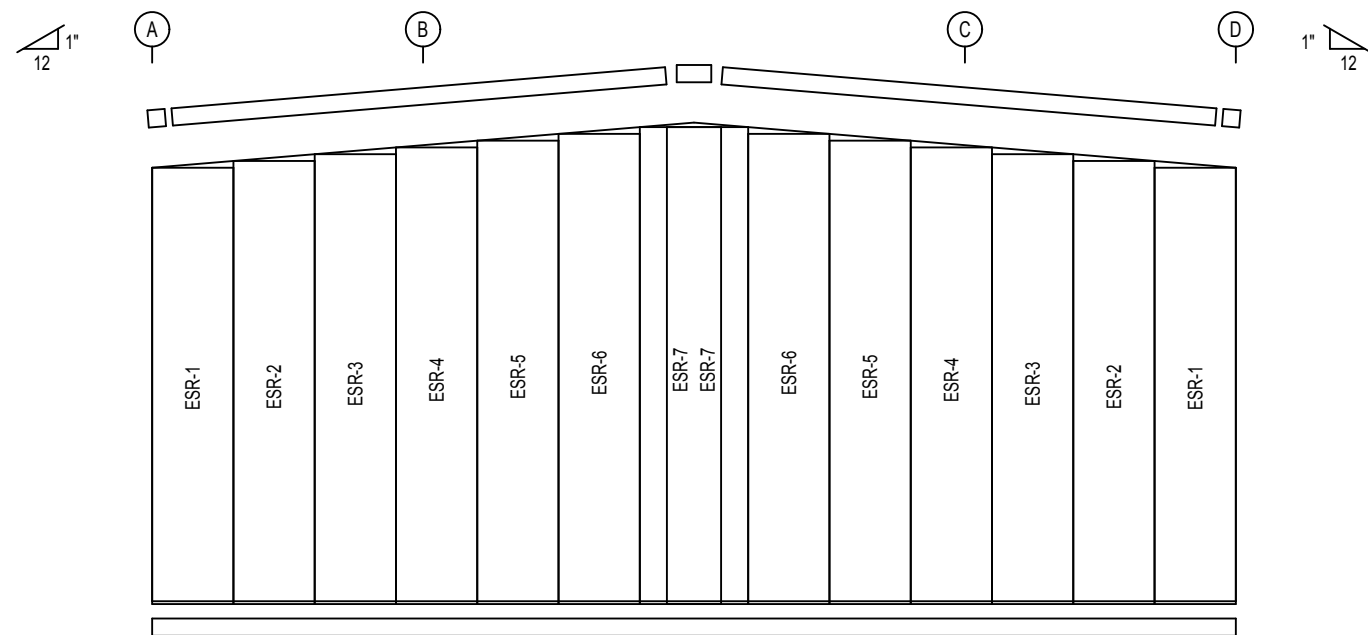
ENDWALL FRAMING: FRAME LINE 3
