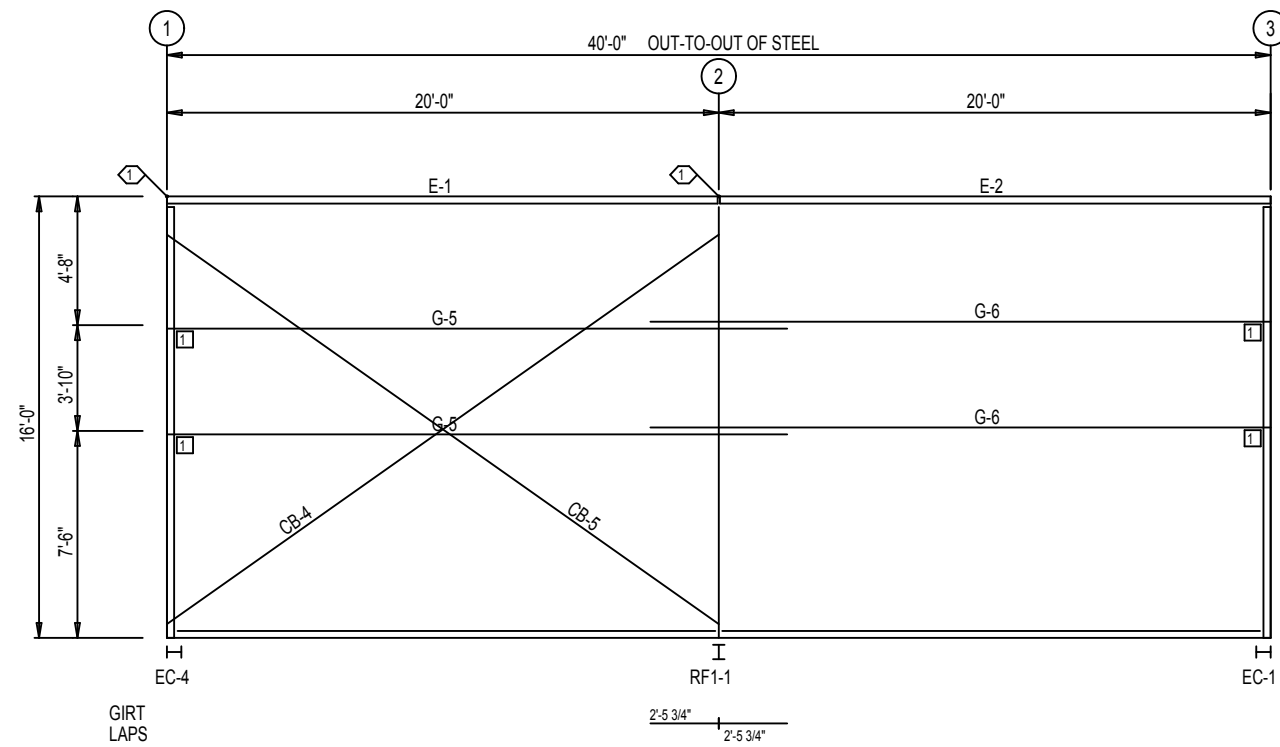
SIDEWALL FRAMING: FRAME LINE A
