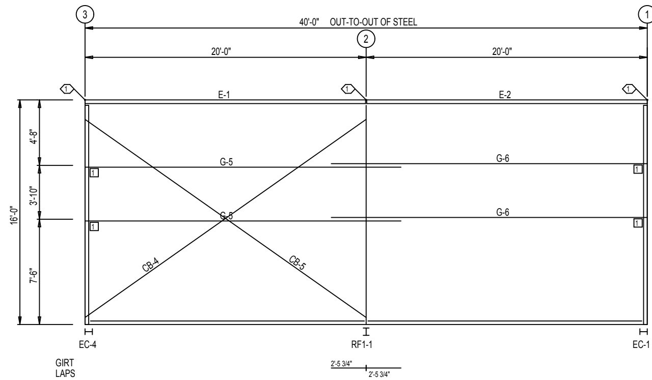
SIDEWALL FRAMING: FRAME LINE D
