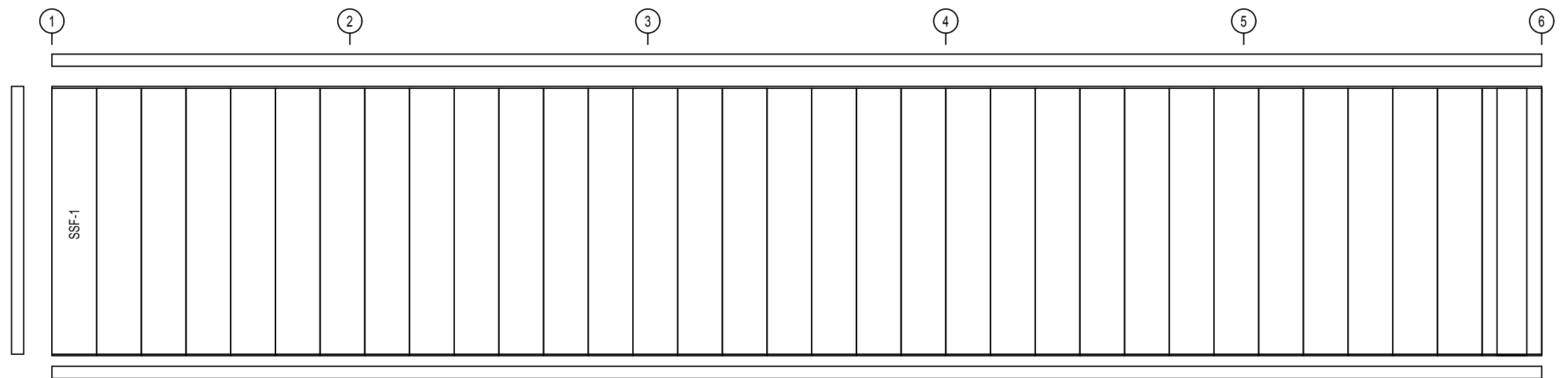
SIDEWALL SHEETING & TRIM: FRAME LINE A
