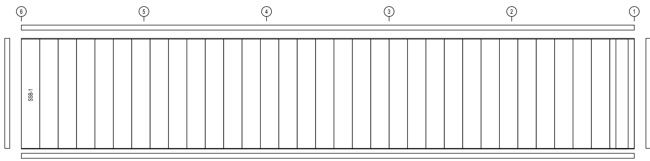
SIDEWALL SHEETING & TRIM: FRAME LINE D PANELS: 26 Gauge PBR - Polar White
