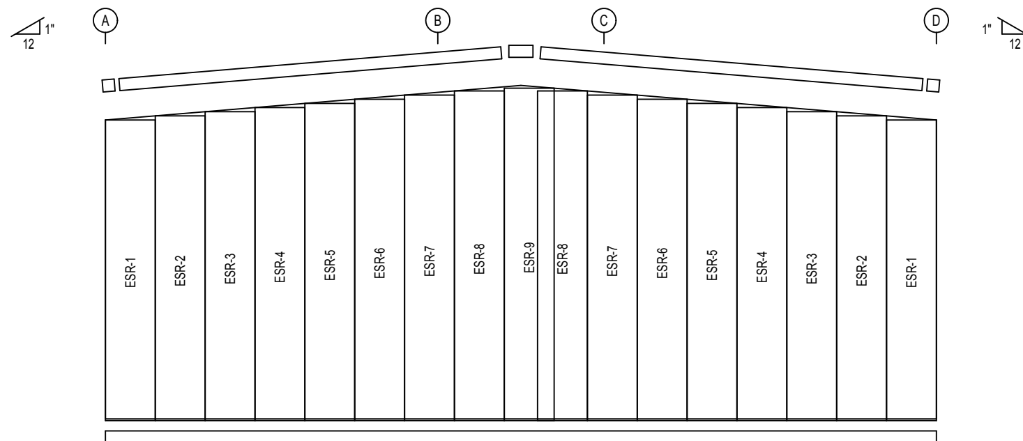
ENDWALL FRAMING: FRAME LINE 6
