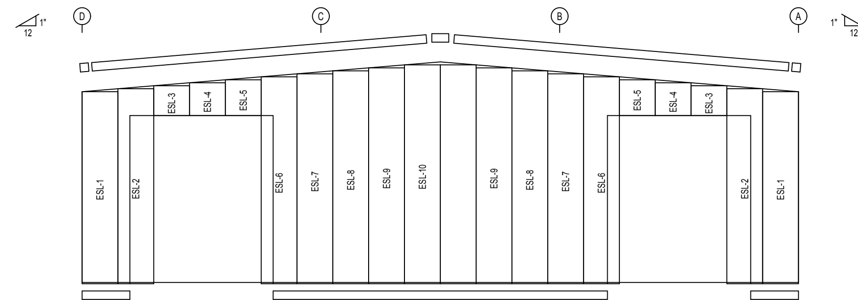
ENDWALL FRAMING: FRAME LINE 1
