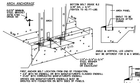
ARCH ANCHORAGE
