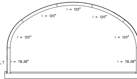
ARCH PROFILE
