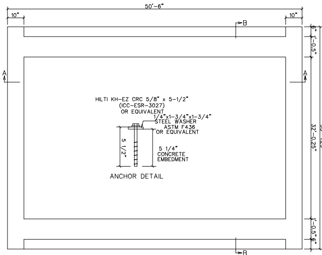
FOUNDATION PLAN
