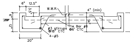
SEC B-B
