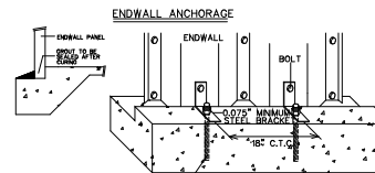
ENDWALL ANCHORAGE
