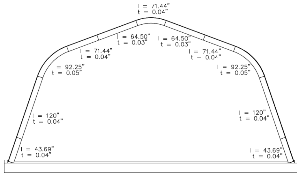
ARCH PROFILE
