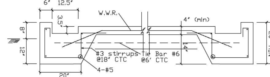
SEC B-B
