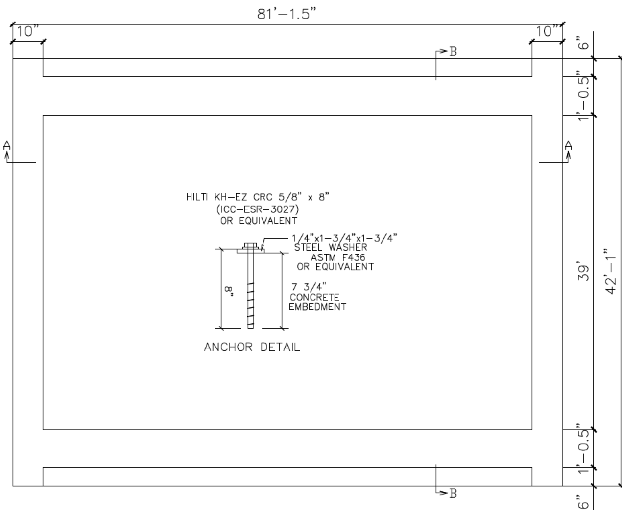
FOUNDATION PLAN
