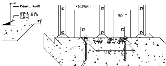
ENDWALL ANCHORAGE
