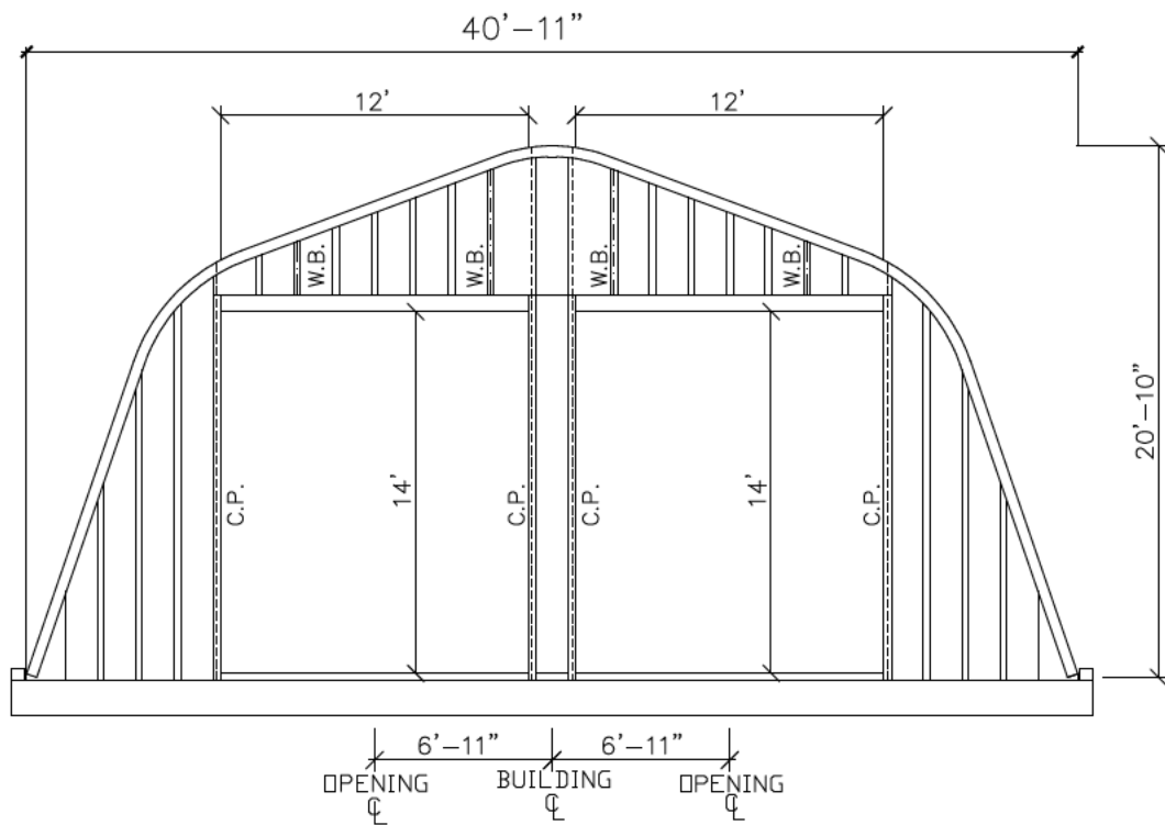
REAR ELEVATION
