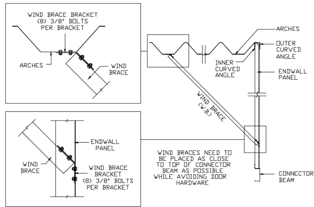
WIND BRACING
