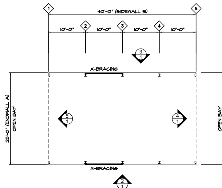
1 BUILDING LAYOUT PLAN 1 SCALE: 1/8" = 1'-0"
