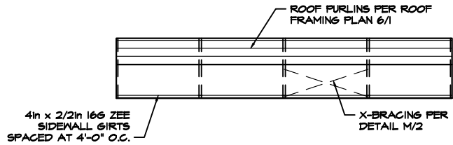
2 SIDEWALL 'A' EXTERIOR ELEVATION 1 SCALE: 1/8" = 1'-0"
