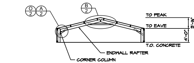
5 ENDWALL 'A' INTERIOR ELEVATION 1 SCALE: 1/8" = 1'-0" FRAME #1
