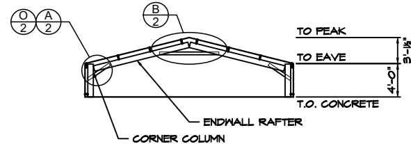
5 ENDWALL 'A' INTERIOR ELEVATION 1 SCALE: 1/8" = 1'-0" FRAME #1
