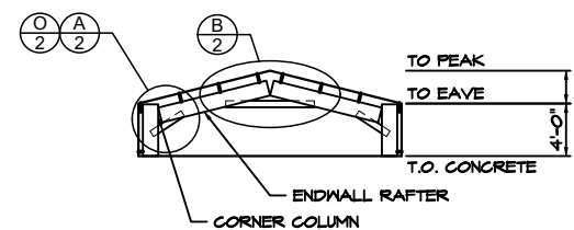
5 1 ENDWALL 'A' INTERIOR ELEVATION SCALE: 1/8" = 1'-0" FRAME #1
