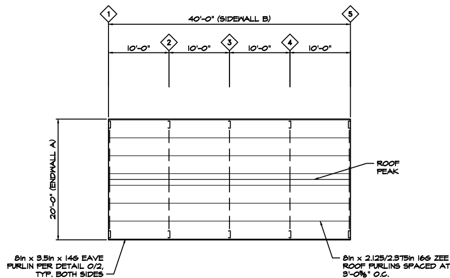
6 1 ROOF FRAMING PLAN SCALE: 1/8" = 1'-0"
