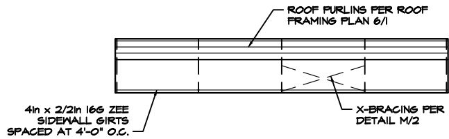
2 1 SIDEWALL 'A' EXTERIOR ELEVATION SCALE: 1/8" = 1'-0"
