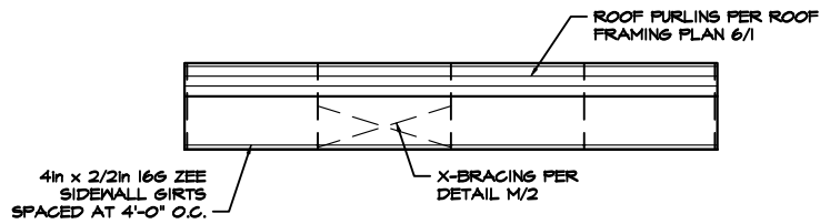
2 1 SIDEWALL 'A' EXTERIOR ELEVATION SCALE: 1/8" = 1'-0"
