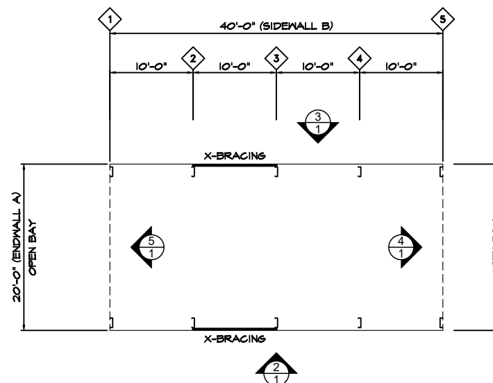
1 1 BUILDING LAYOUT PLAN SCALE: 1/8" = 1'-0"
